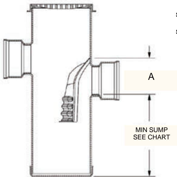
Structure Side View
